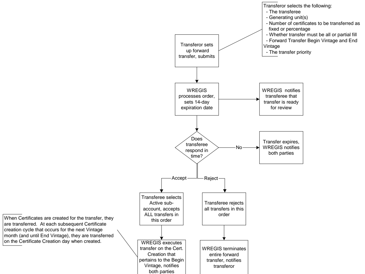
Figure 6: Flowchart showing Forward Certificate Transfer
